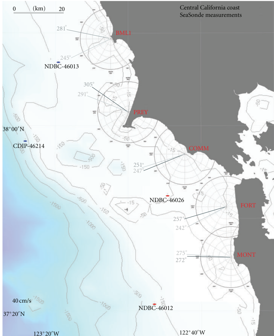
FIGURE 16: Annual mean wave directions for 2007 calculated from SeaSonde wave data (dark grey) and near-shore CDIP model annual mean wave direction results (light grey).
