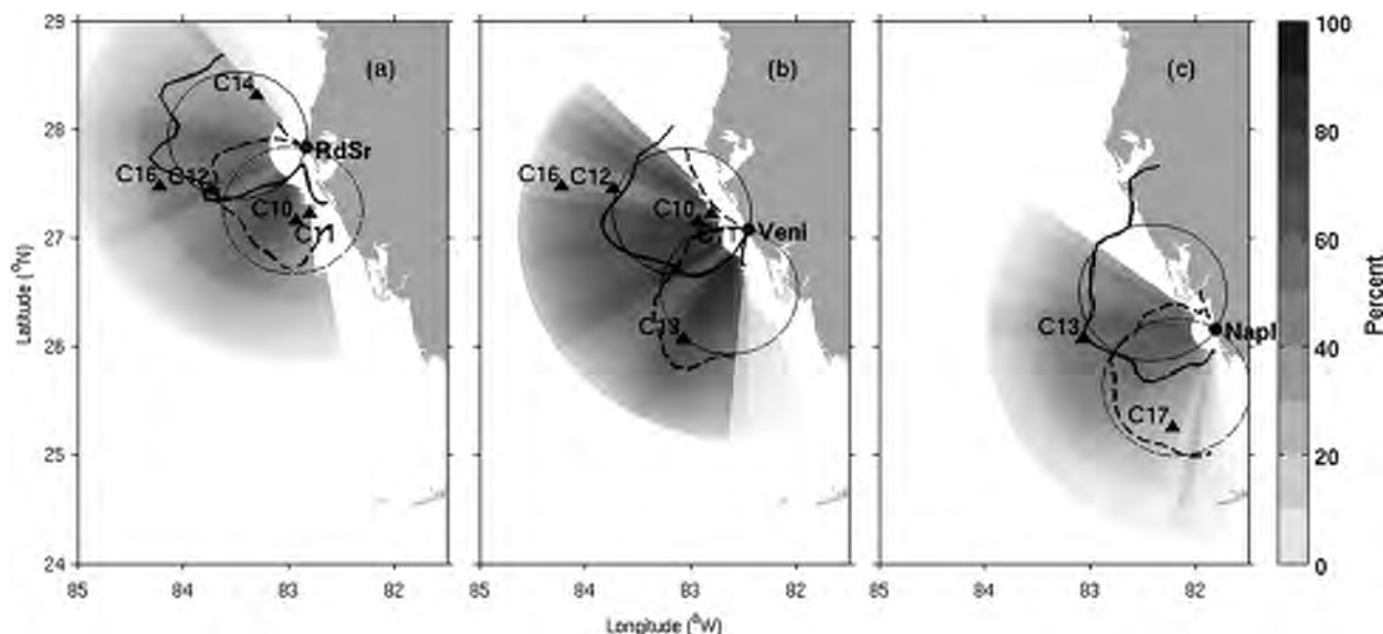
FIG. 6. Percent temporal coverage of valid radial currents for the three HF radar sites: (a) Redington Shores (RdSr), (b) Venice (Ven), and (c) Naples (Napl). Measured antenna patterns are superimposed [black bold lines; loops 1–3 (solid) and loops 2 and 3 (dashed)] and ideal antenna patterns are shown (thin dashed lines). The ADCP stations (solid triangles) for comparison are shown for each HF radar site.
