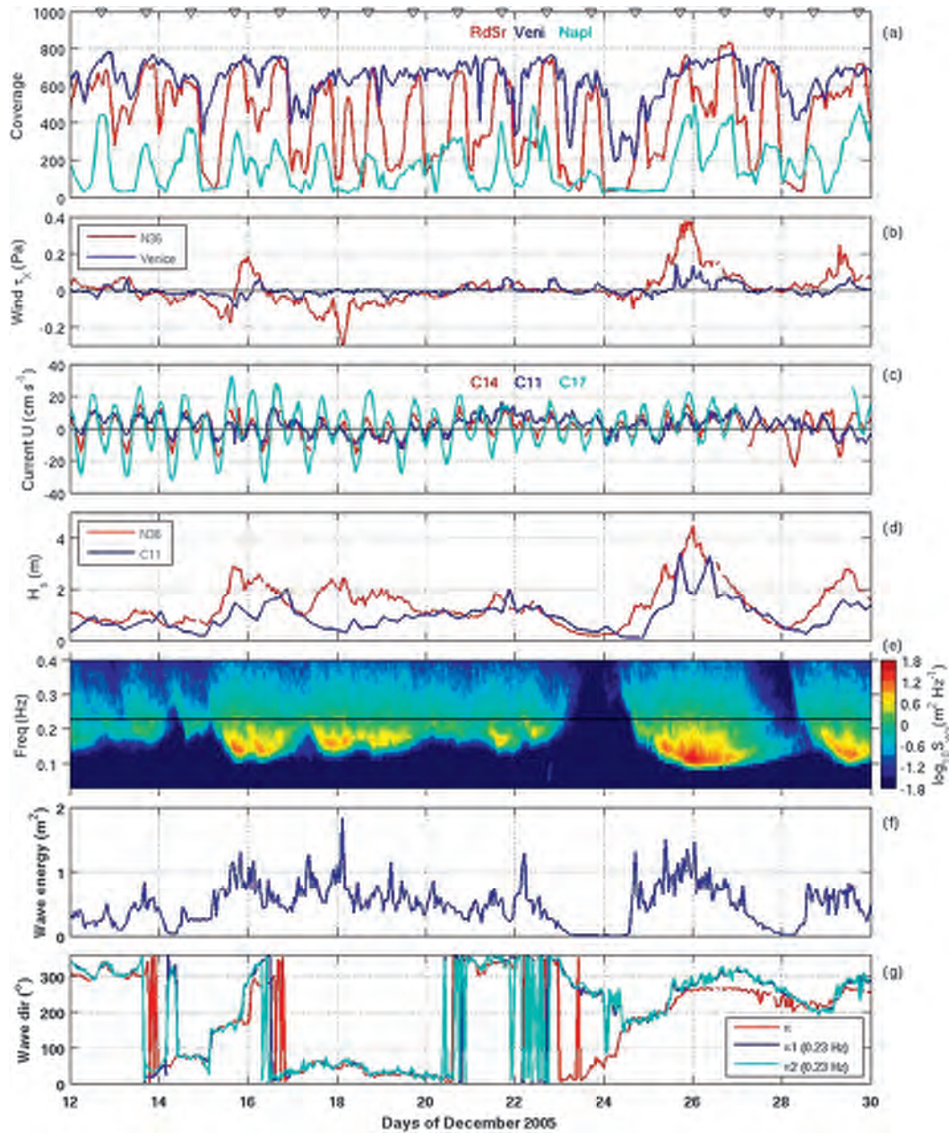
FIG. 3. Time series of (a) radial coverage from the three HF radar sites, Redington Shores (RdSr), Venice (Veni), and Naples (Napt), Florida; (b) wind east–west component at NDBC buoy 42036 and Venice; (c) surface current east–west component at moorings C14, C11, and C17; (d) significant wave height ( H_s ) observed at NDBC buoy 42036 and University of South Florida (USF) College of Marine Science mooring C11; (e) spectral wave energy at NDBC buoy 42036 (solid line indicates frequency of 0.23 Hz); (f) wave energy at frequency of 0.23 Hz; and (g) wave directions are measured from true north increase clockwise ( 0^\circ = north, 90^\circ = east): the direction from which the waves at the dominant period are coming ( \alpha ), the mean ( \alpha_1 ), and the principal wave directions ( \alpha_2 ) at frequency of 0.23 Hz. The sampling intervals are 1 h for all the time series except the significant wave height at mooring C11, which was sampled every 4 h. The upside-down triangles on the top panel indicate local noon.
