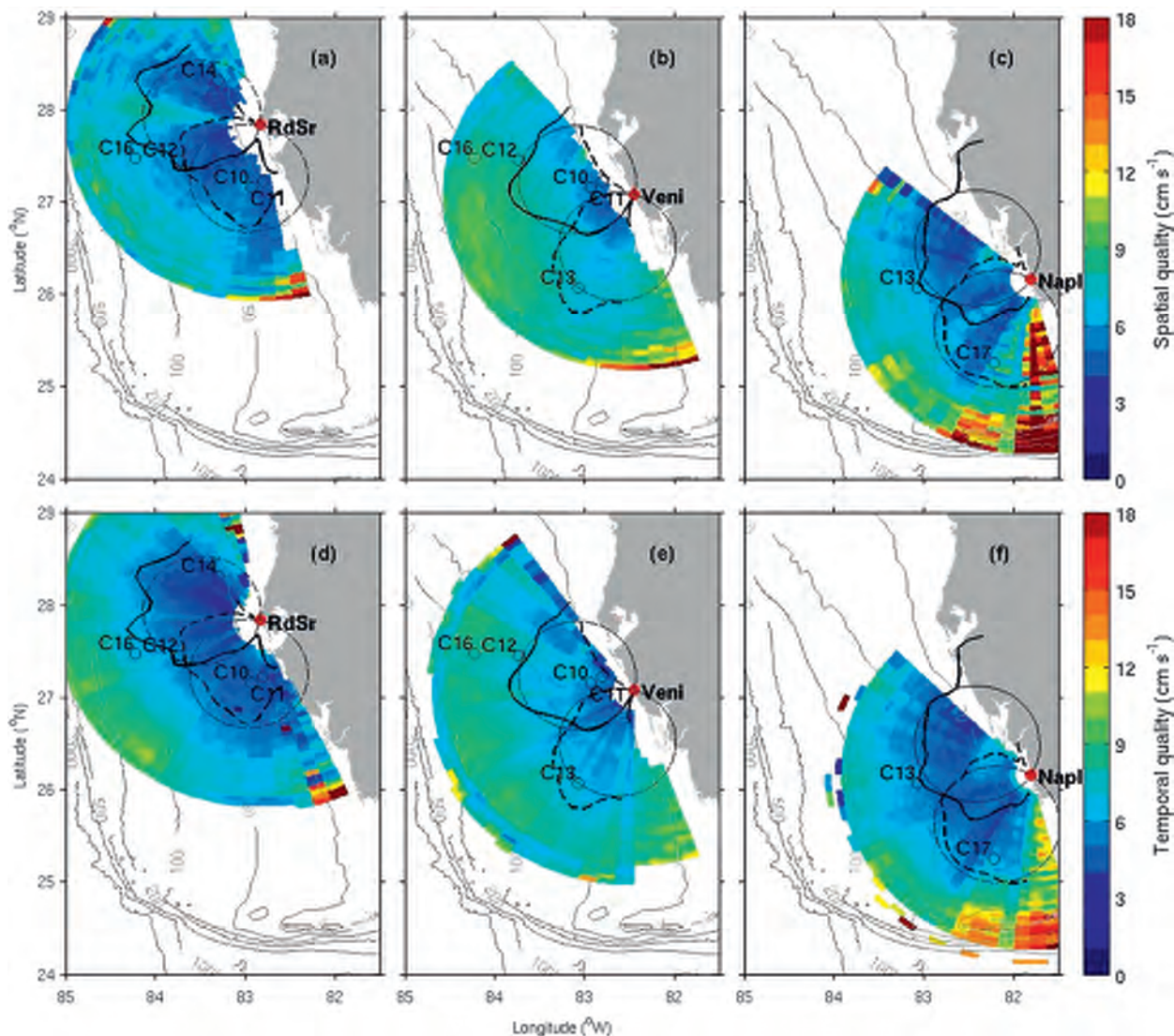
FIG. 14. Record-long mean (top) spatial and (bottom) temporal quality factors (or uncertainties) of the radial currents for each range-bearing cell of the three HF radar sites: (a),(d) Redington Shores (RdSr), (b),(e) Venice (Veni), and (c),(f) Naples (Napl). Measured antenna patterns are superimposed [black bold lines; loops 1–3 (solid) and loops 2 and 3 (dashed)], and ideal antenna patterns are shown (thin dashed lines). The ADCP stations (solid triangles) for comparison are shown for each HF radar site. The idealized antenna pattern was used prior to the measured beam pattern was available.
