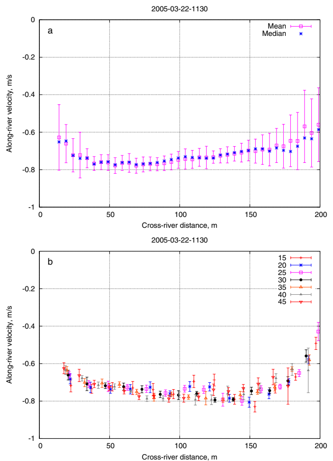
Fig. 3. Along-channel RiverSonde velocity vs distance across the channel for 22 March 2005 at 11:30 at Threemile Slough. The distance origin is at the radar antenna, and positive velocity represents flow toward the north. The blue asterisks show the median of 9 measurements taken over a 15-minute interval, and the red symbols show the sample means and standard deviations of the same measurements. (a) Profile calculated by fitting a vector to all the radials falling within a 5-m strip parallel to the flow direction. Velocity estimates are made every 5 m across the 200-m wide channel. (b) Profile calculated by combining radial vectors in 5^\circ sectors symmetrically displaced from the perpendicular to the flow direction.
