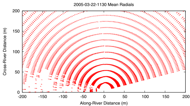
Fig. 2. Radial flow vectors averaged over 15 minutes on 22 March 2005 at 11:30 PST at Threemile Slough. Vectors are plotted between the river banks with 1^\circ resolution in angle and 15 m in range. A velocity of 1.0 m/s is plotted with an equivalent length of 10 m. The mean direction of flow is aligned with the horizontal axis, with north toward the left. The broadside direction of the antenna is about 12^\circ counterclockwise from the perpendicular direction to the bank, and the sharp angular cutoff at the right side of the plot is due to antenna hardware and data processing limitations.
