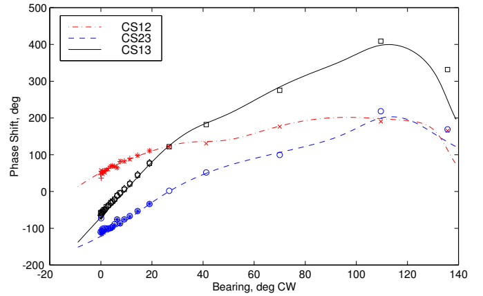
Fig. 4. Phase calibration at Vernalis. Lines are NEC predictions, points are measured values. The NEC predictions have been shifted vertically to account for cable delays in order to best match the measurements, but their shape is unchanged. CS12, CS23, CS13 refer to the phases of the cross-spectra between antennas 1&2, 2&3, and 1&3, respectively. Antennas are numbered as in Fig. 1. The transponder was carried on a cable stretched across the river, so measurements tend to cluster near broadside at the far bank.
