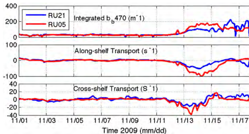
Fig. 12. Time-series of the (blue) RU21 and (red) RU05 (top) three-hour integrated b_{470} ( m^{-1} ) and estimated transport in the (middle) along- and (bottom) cross- shelf directions. Positive values indicate northeastward transport for along-shelf and southeastward transport for cross-shelf transport. Estimated transport is calculated by multiplying depth-averaged glider currents by integrated optical backscatter at b_{470} .
