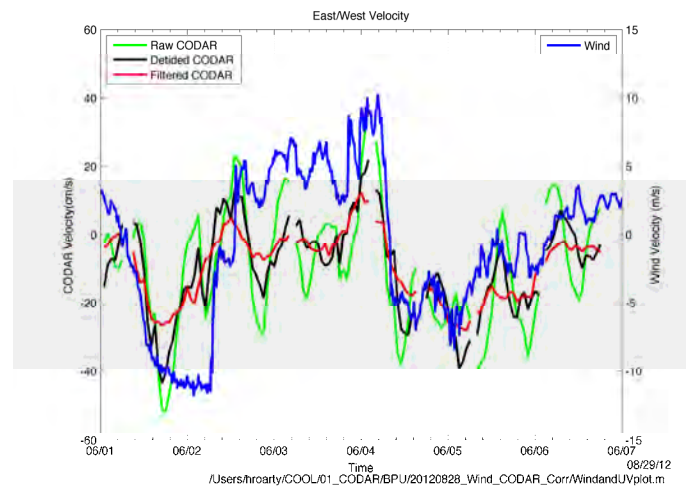
Figure 2: Time series plot from June 1-7, 2012 of the u velocity of the CODAR surface currents (green), detided surface currents (black), low pass filtered currents (red) and wind from station 44025 (blue).
