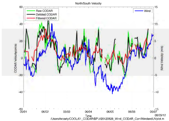
Figure 3: Time series plot from June 1-7, 2012 of the v velocity of the CODAR surface currents (green), detided surface currents (black), low pass filtered currents (red) and wind from station 44025 (blue).
