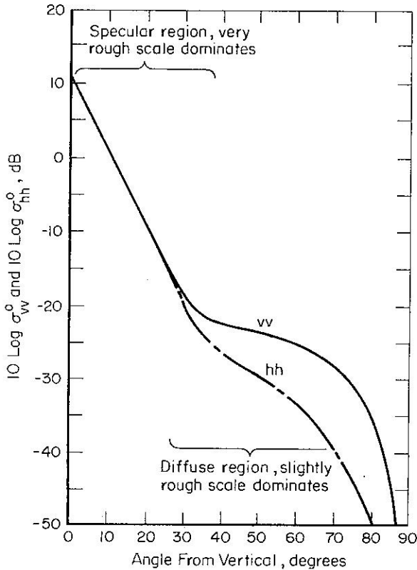
FIGURE 2. Theoretical curves for backscattering cross section per unit area of composite surface having a dielectric constant \epsilon_r=5.0 for vertical and horizontal polarization states.
